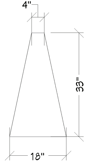
18" wedge
